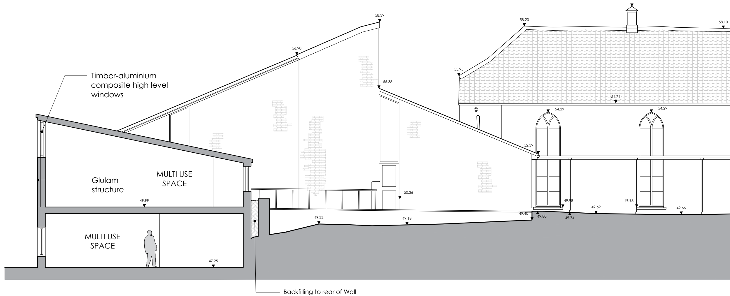
Proposed Section C-C 1:100
